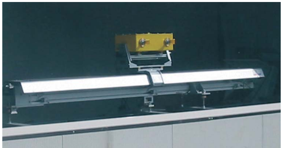
Fig.5 - Vista frontale dell'interferometro SAR terrestre modello IBIS-L - Front view of ground-based SAR interferometer model IBIS-L
